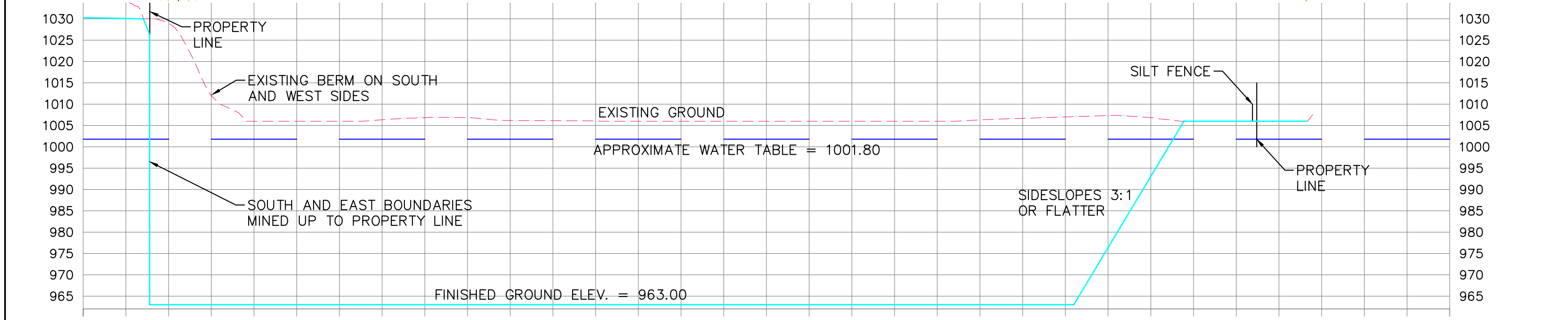
SECTION A - A
