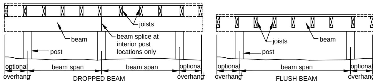
Figure 3 BEAM TYPES
