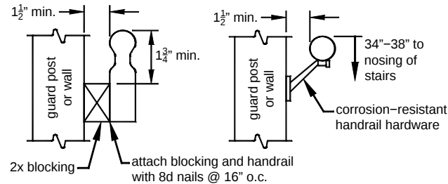
Figure 34 HANDRAIL GRASPABILITY
