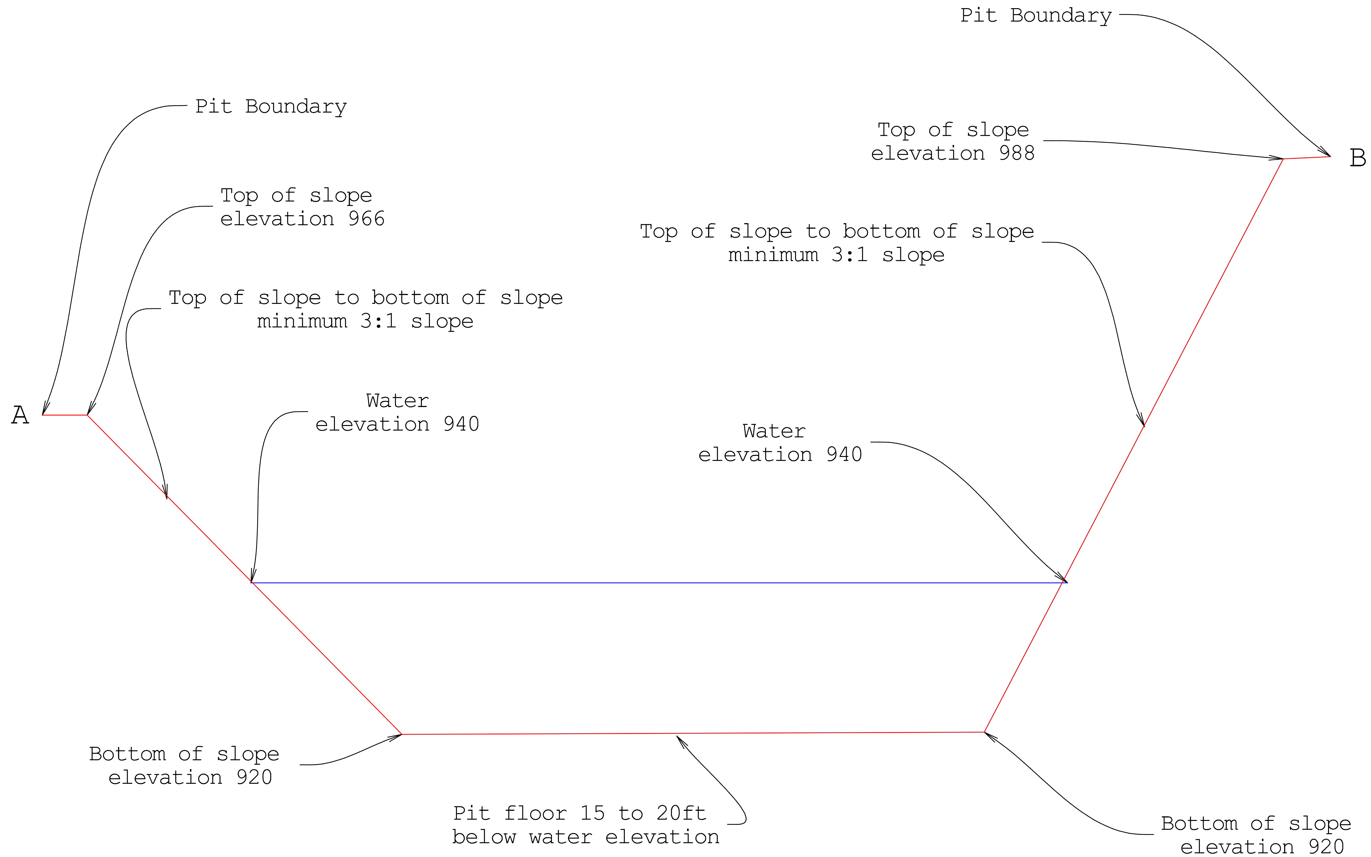
Mallard Road Cross Section A-B
