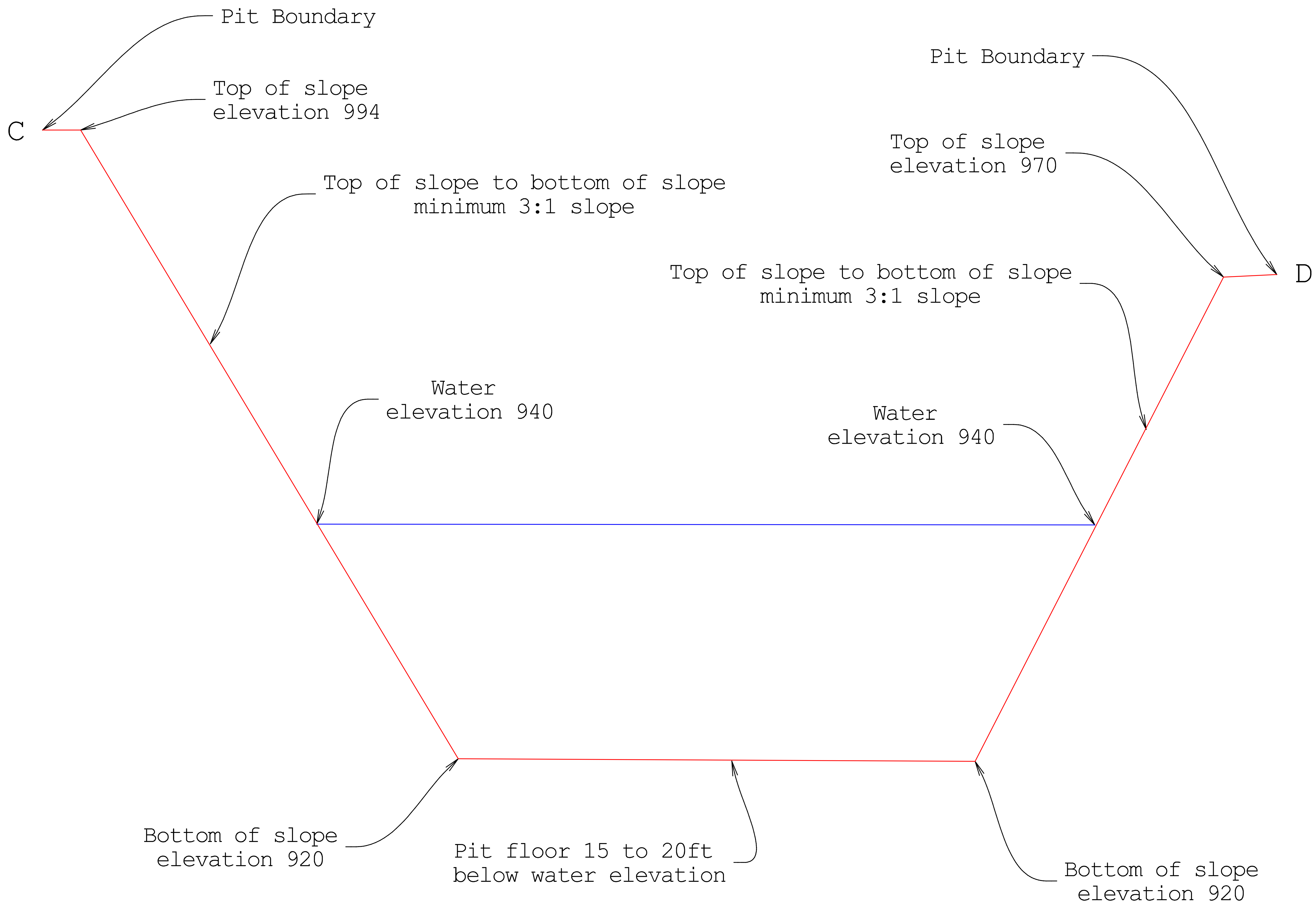
Mallard Road Cross Section C-D
